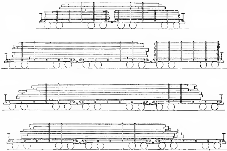
Figs. 5573-5576. RECOMMENDED PRACTICE FOR LOADING POLES AND LOGS. The lines across Stakes indicate Ties across Cars.
